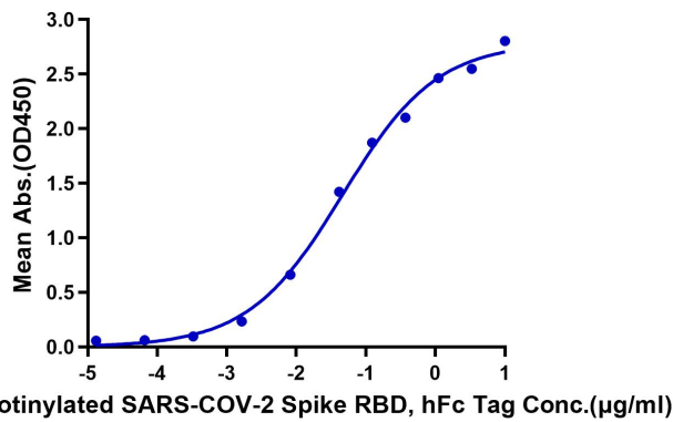
Human ACE2, His Tag ELISA 0.5µg Human ACE2, His Tag Per Well
